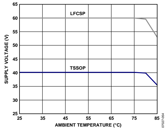
Figure 52. Maximum Supply Voltage vs. Ambient Temperature
