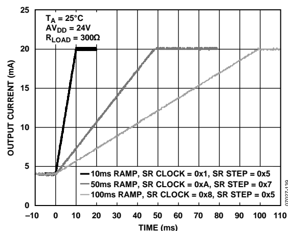
Figure 41. Output Current Slewing Under Control of the Digital Slew Rate Control Feature
