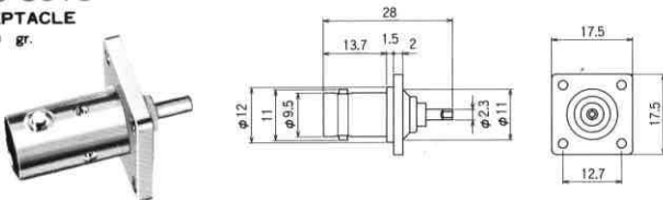
No. MNC-601L RIGHT ANGLE BNC RECEPTACLE Net Weight: 14 gr
