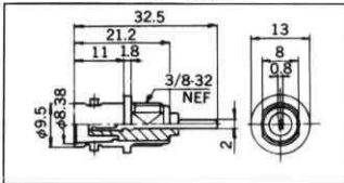
No. MNC-601SW BNC RECEPTACLE W/SWITCH
