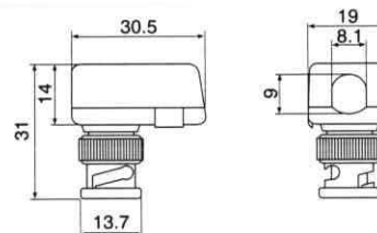
No.MTV-226BL SHIELDED BNC PLUG RIGHT ANGLE TYPE
