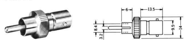
No. MNC-542 RCA TO BNC JACK
