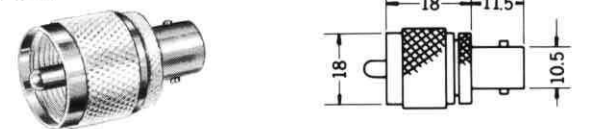
No. MNC-580 PL-259 TO BNC JACK. Net Weight: 24 gr.
