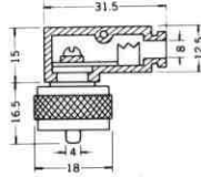
No. MR-586LS RIGHT ANGLE UHF PLUG (PL-259) SOLDERLESS TYPE Net Weight: 16 gr.
