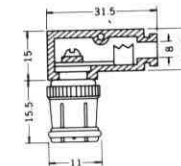
No. MR-556LS RIGHT ANGLE F TYPE QUICK PLUG SOLDERLESS TYPE Net Weight: 10 gr.
