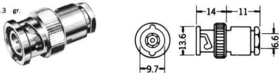
No. MNC-577 BNC PLUG TO F JACK. Net Weight: 15 gr.
