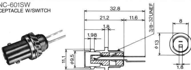
No. MNC-601S BNC RECEPTACLE Net Weight: 9 gr.
