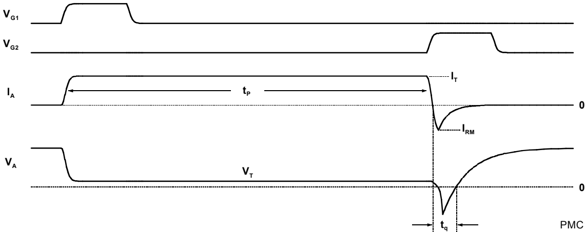
Figure 2. Circuit-commutated turn-off time
