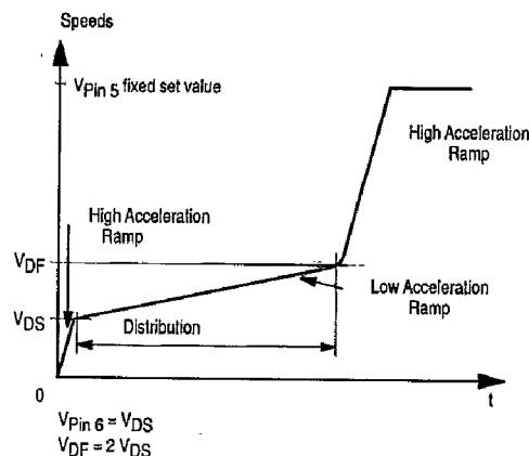
Figure 3. Programmable Double Acceleration Ramp
