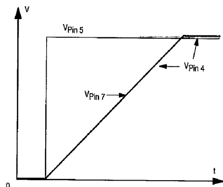
Figure 2. Acceleration Ramp
