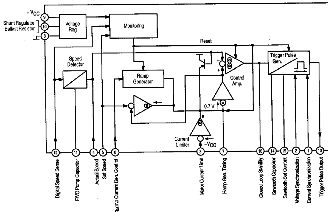
Figure 1. Representative Block Diagram and Pin Connections
