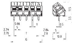
without insulating plate
