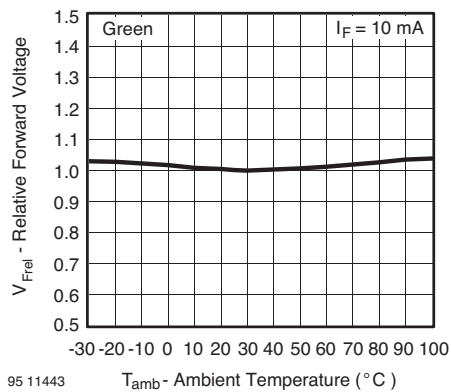
Figure 21. Relative Forward Voltage vs. Ambient Temperature
