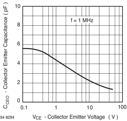
Figure 6. Collector Emitter Capacitance vs. Collector Emitter Voltage
