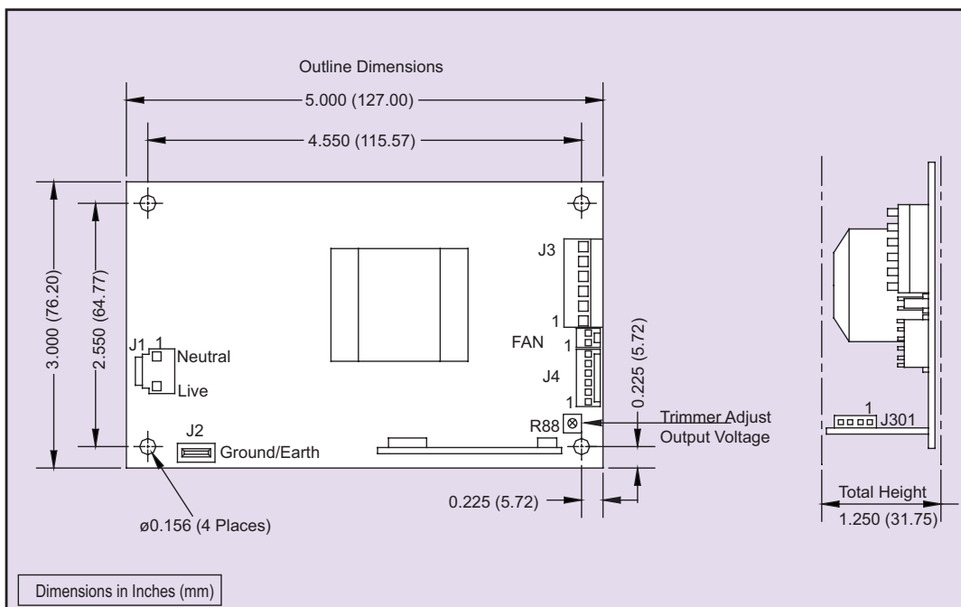
Figure 2: Mechanical Drawing
