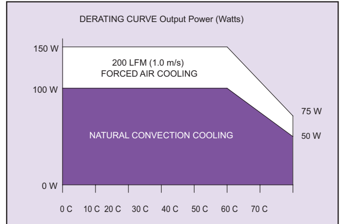
Figure 1: Derating Curve
