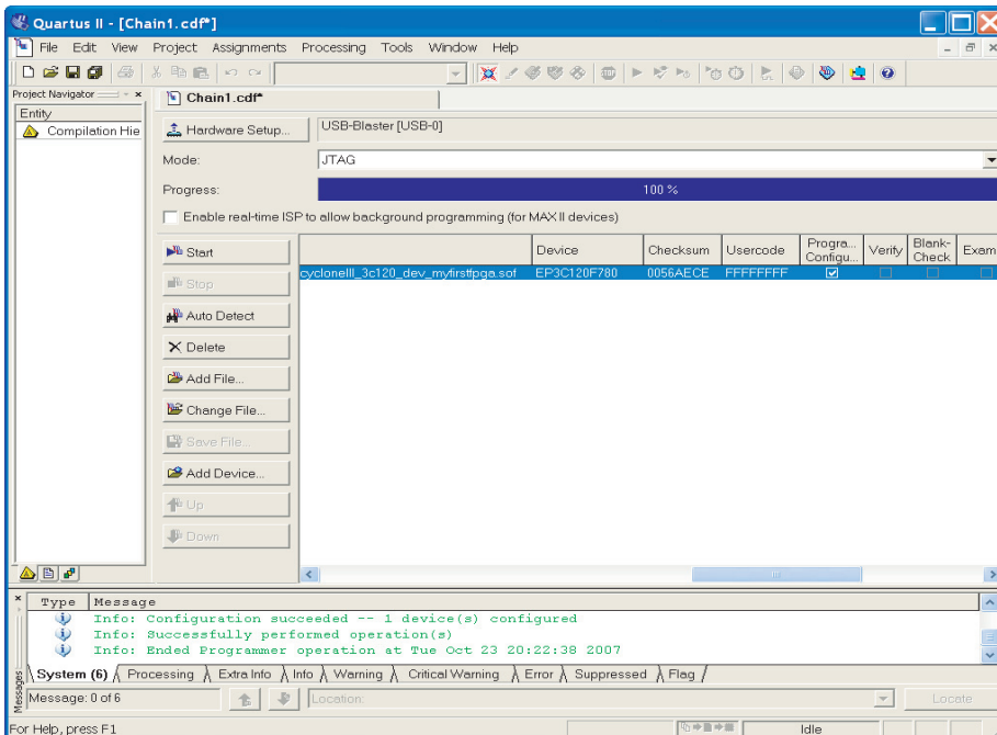
Figure 4–2. Quartus II Programmer
