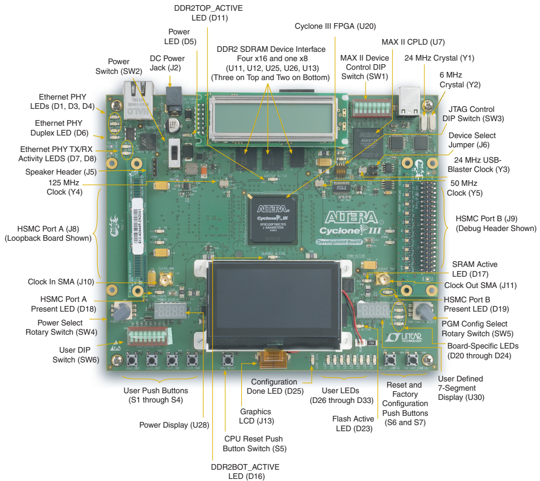
Figure 4–1. Cyclone III Development Board Layout and Components
