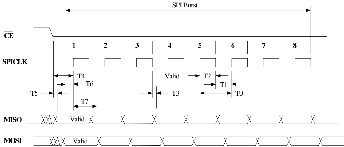
Figure 8. SPI Single Burst Timing Diagram
