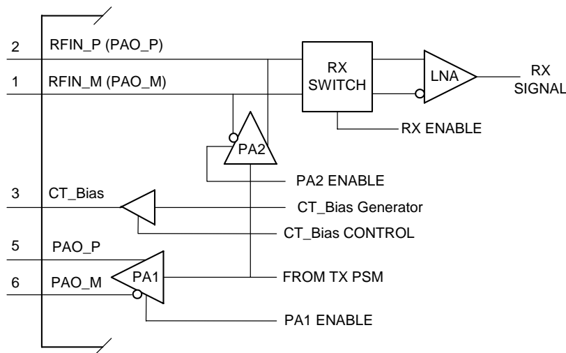
Figure 12. RF Interface Pins
