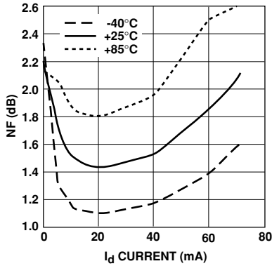
Figure 15. Minimum Noise Figure vs. Current and Temperature.
