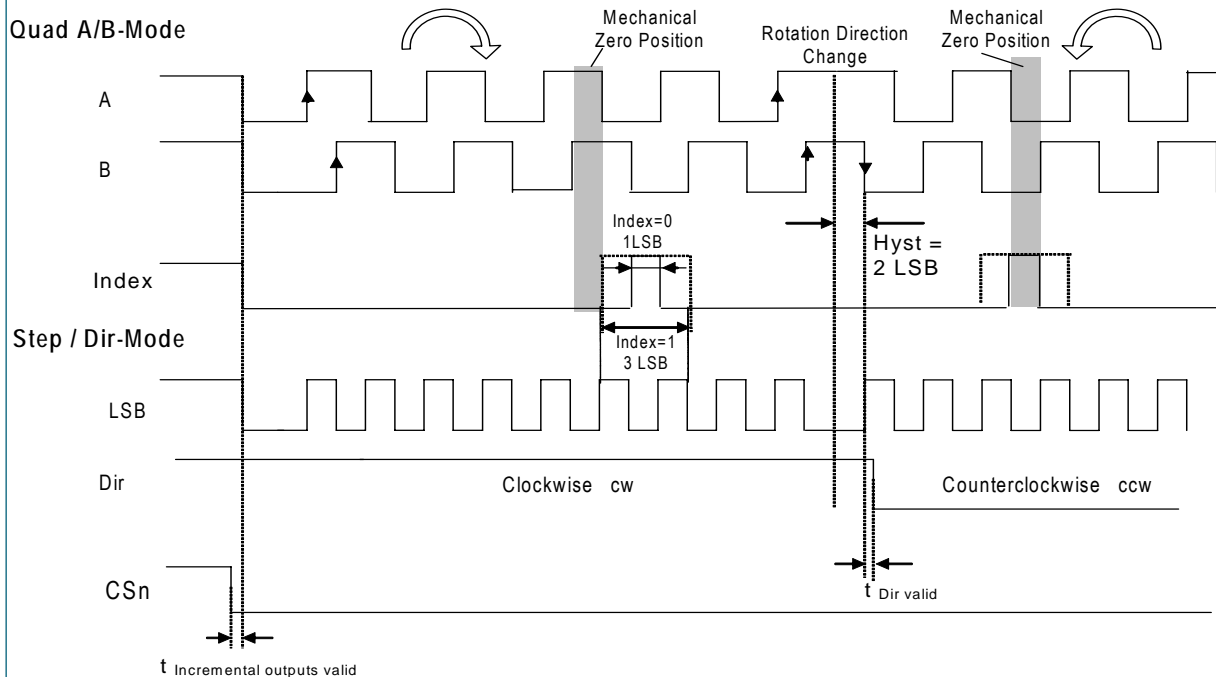
Figure 8: Incremental output modes
