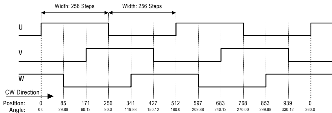
Figure 13: U, V and W-signals for 2pole BLDC motor commutation (Div1=1; Div0=0)
