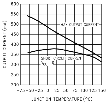
Short-Circuit Output Current and Maximum Output Current
