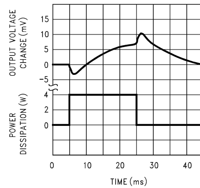
Thermal Response
