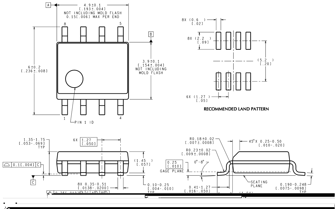
SO-8 Surface Mount Package Order Number LP2954AIM or LP2954IM NS Package Number M08A
