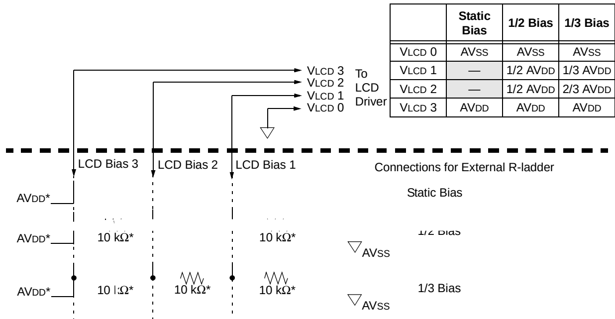
FIGURE 22-3: LCD BIAS RESISTOR LADDER CONNECTION DIAGRAM
