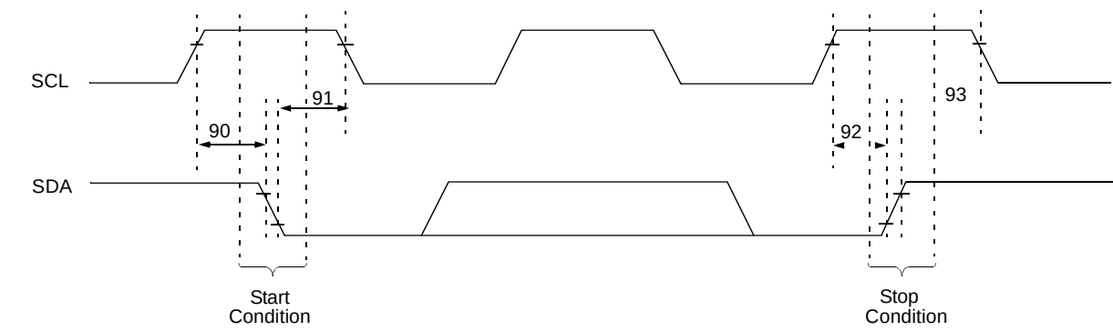
FIGURE 26-17: MASTER SSP I 2 C™ BUS START/STOP BITS TIMING WAVEFORMS
