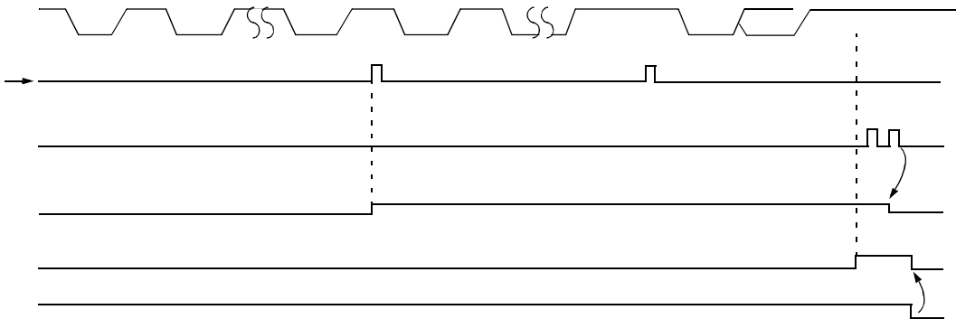
FIGURE 16-7: ASYNCHRONOUS RECEPTION
