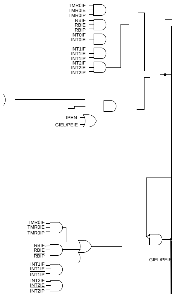
FIGURE 8-1: PIC18F6X90/8X90 INTERRUPT LOGIC
