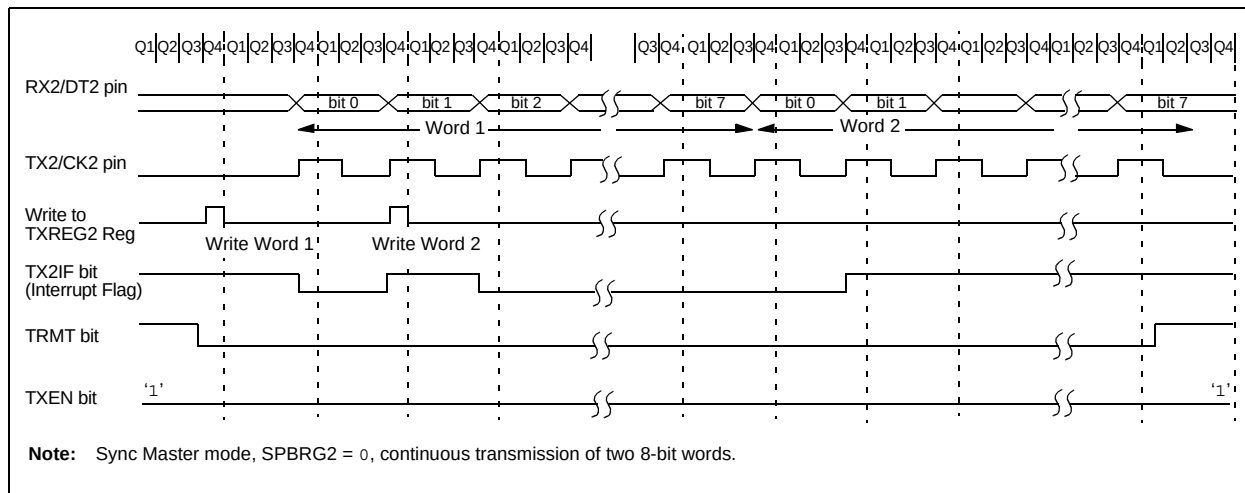
FIGURE 17-6: SYNCHRONOUS TRANSMISSION
