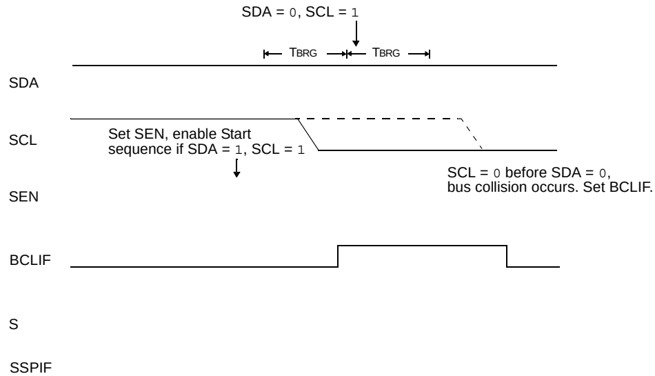
FIGURE 15-27: BUS COLLISION DURING START CONDITION (SCL = 0)
