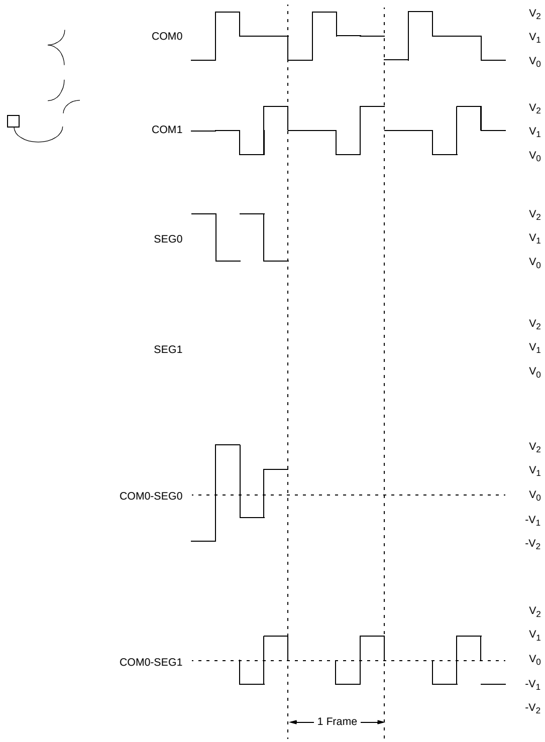
FIGURE 22-5: TYPE-A WAVEFORMS IN 1/2 MUX, 1/2 BIAS DRIVE
