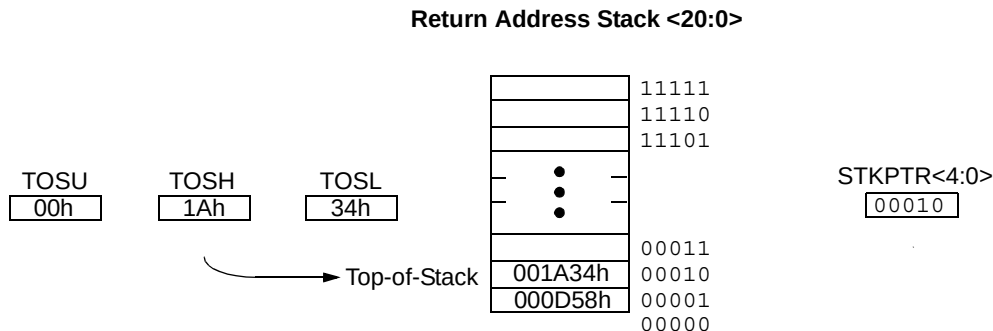
FIGURE 5-2: RETURN ADDRESS STACK AND ASSOCIATED REGISTERS
