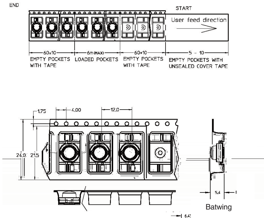
Figure 10. Tape dimensions for Batwing radiation pattern.
