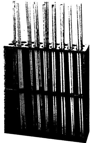
MODEL 367* Threaded Rod Rack. Separates and protects threaded rods. Eighteen 2 1/8" diameter openings accommodate different sizes. Shipped fully assembled.
