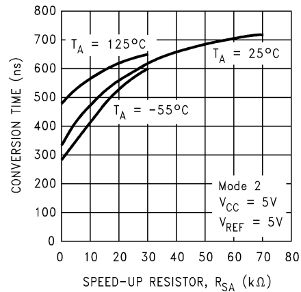
Conversion Time vs. Speed-Up Resistor
