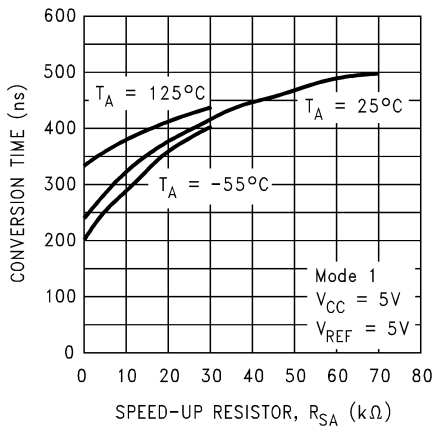
Conversion Time vs. Speed-Up Resistor
