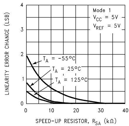
Linearity Change vs. Speed-Up Resistor
