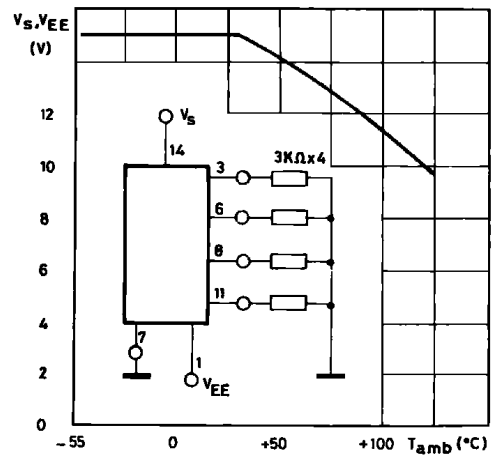
Figure 11 : Maximum Operating Temperature vs Power Supply Voltage
