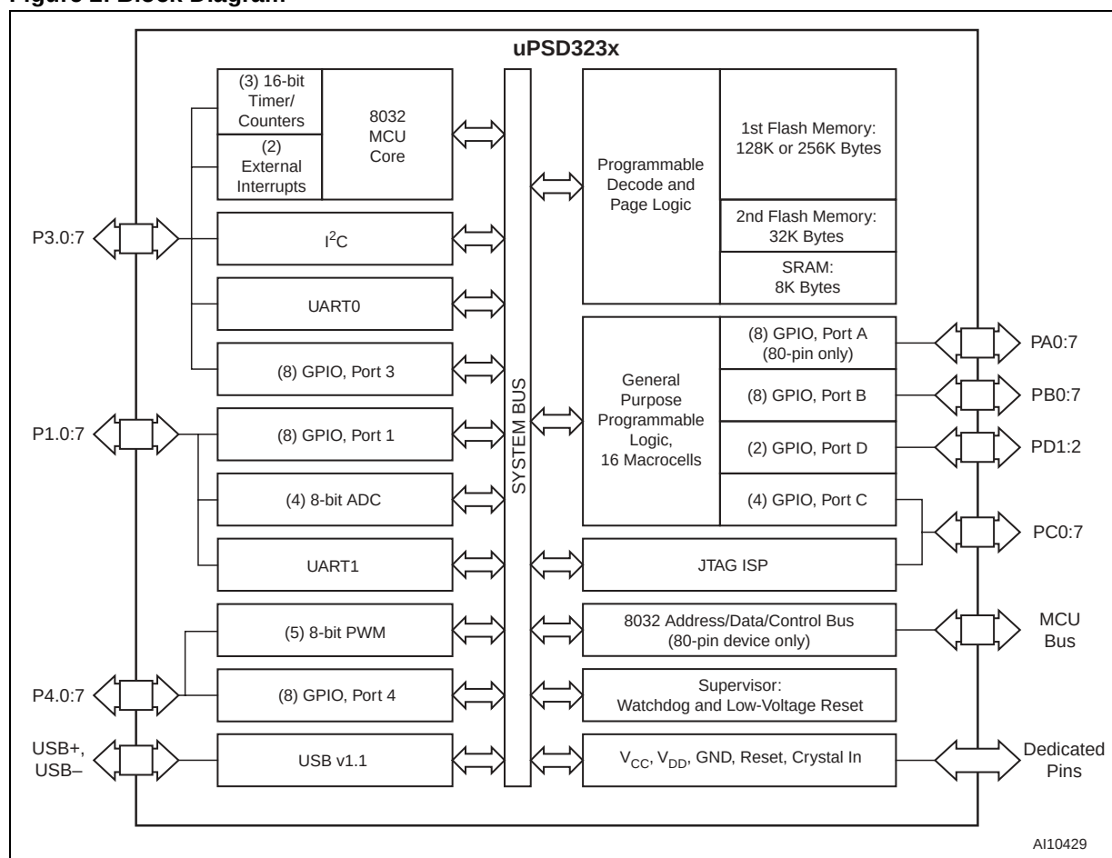
Figure 2. Block Diagram
