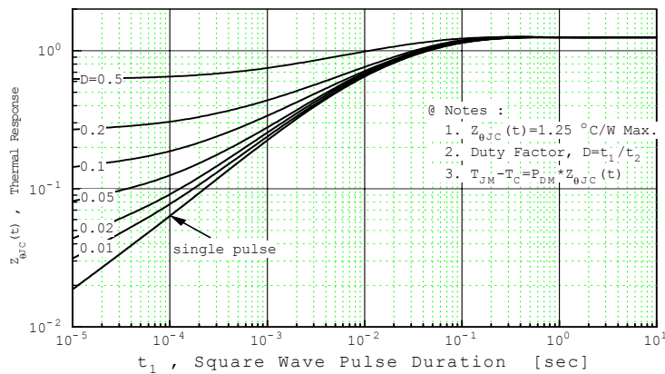
Figure 11. Thermal Response
