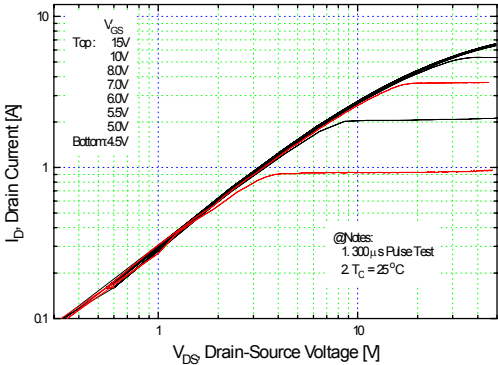
Figure 1. Output Characteristics
