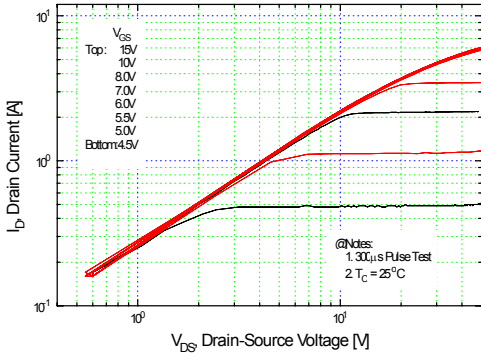
Figure 1. Output Characteristics
