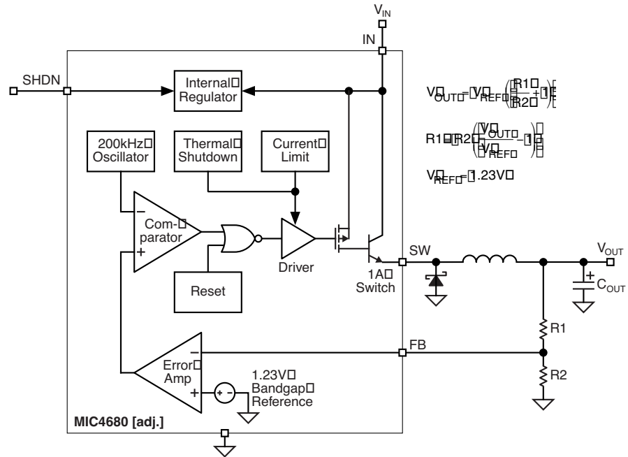
Adjustable Regulator
