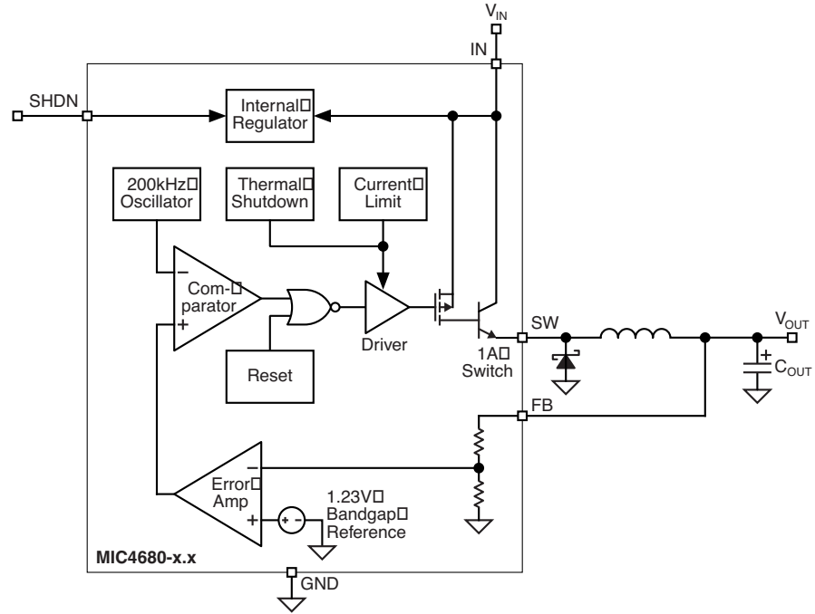
Fixed Regulator
