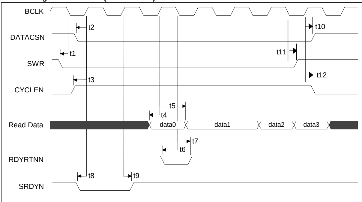
Figure 21. Synchronous Burst Read Cycles – VLBSN = 1
