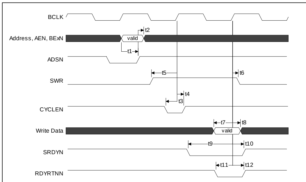
Figure 22. Synchronous Write Cycle – VLBSN = 0
