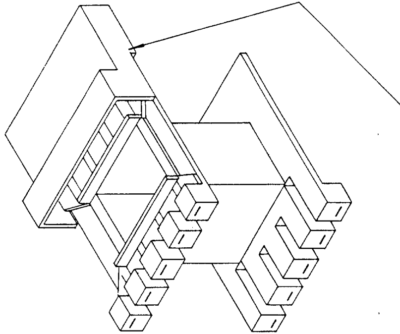
Insulator fitted to one bobbin cheek
