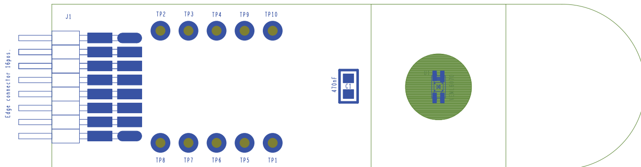
Assembly top
